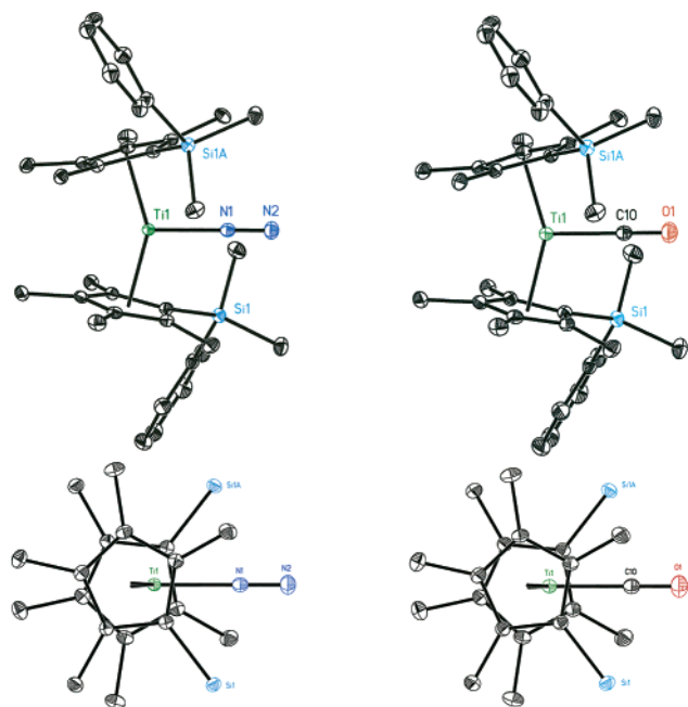
Figure 1. Molecular structures of 2-N 2 (left) and 2-CO (right) at 30% probability ellipsoids with top views shown below. Hydrogen atoms and silyl substituents in the top views are omitted for clarity.
